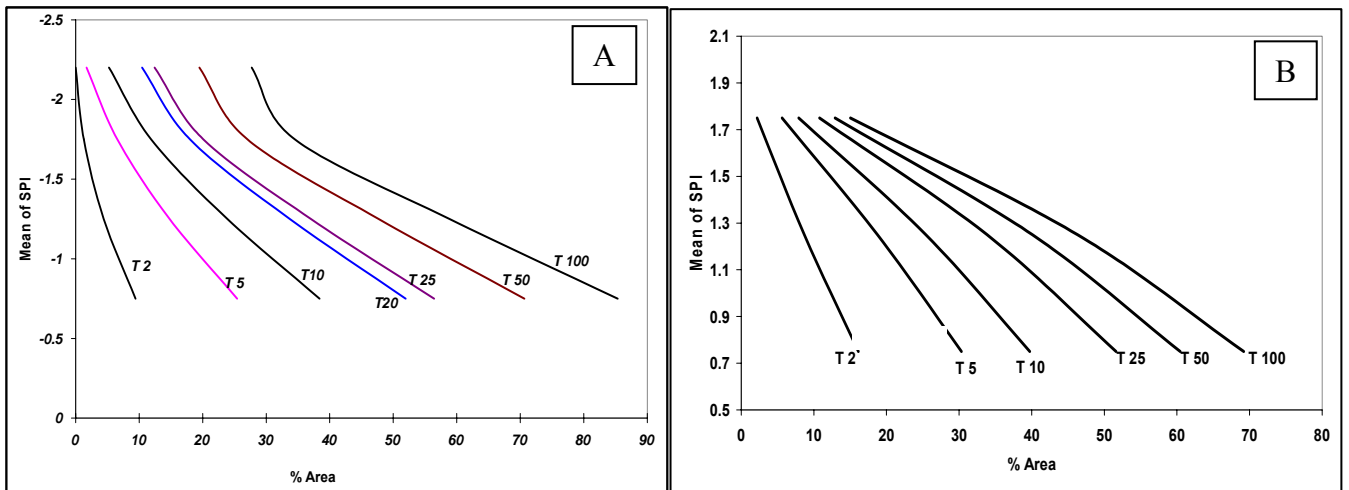
Figure 7: SAF diagram in Razavi and South Khorasan A) for drought, B) for wet
