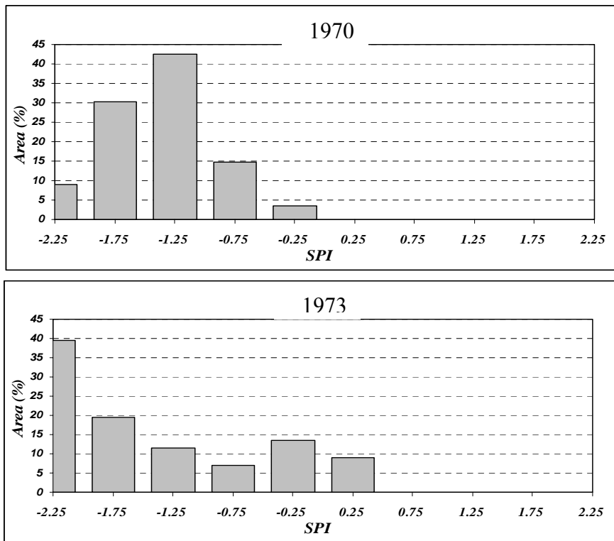
Figure 5: percentage of each SPI category in 1970 (top) and 1973 (bottom).
