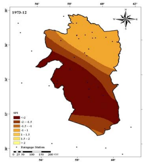
Figure 4: september 1973 drought map
