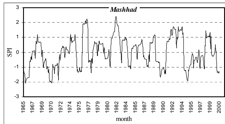
Figure 2: 12-month September SPI 1965-2000 time series for Mashhad station
