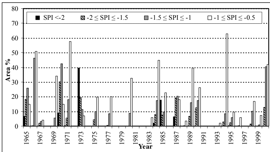
Figure 6: percentage area covered by droughts of different SPI severity
