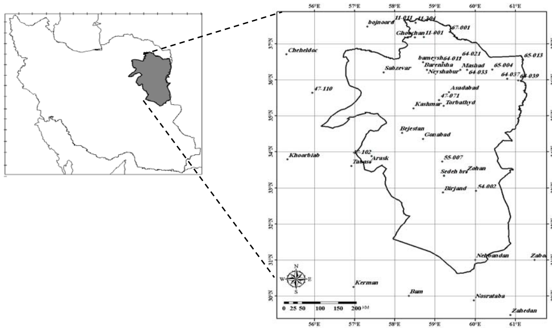
Figure 1: study area and the distributions of the rain stations
