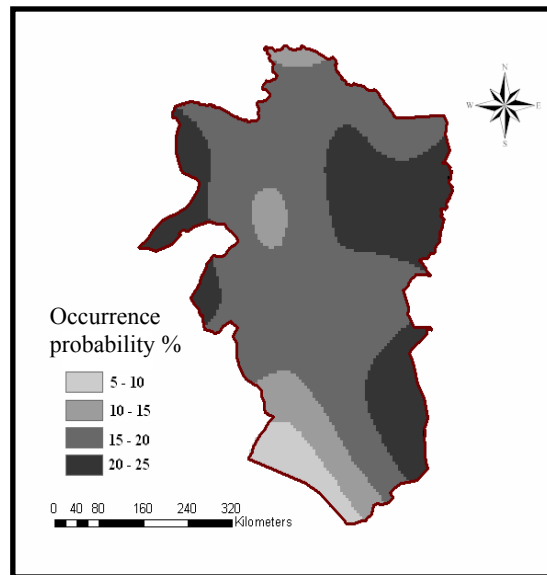
Figure 8. drought occurrence probability
